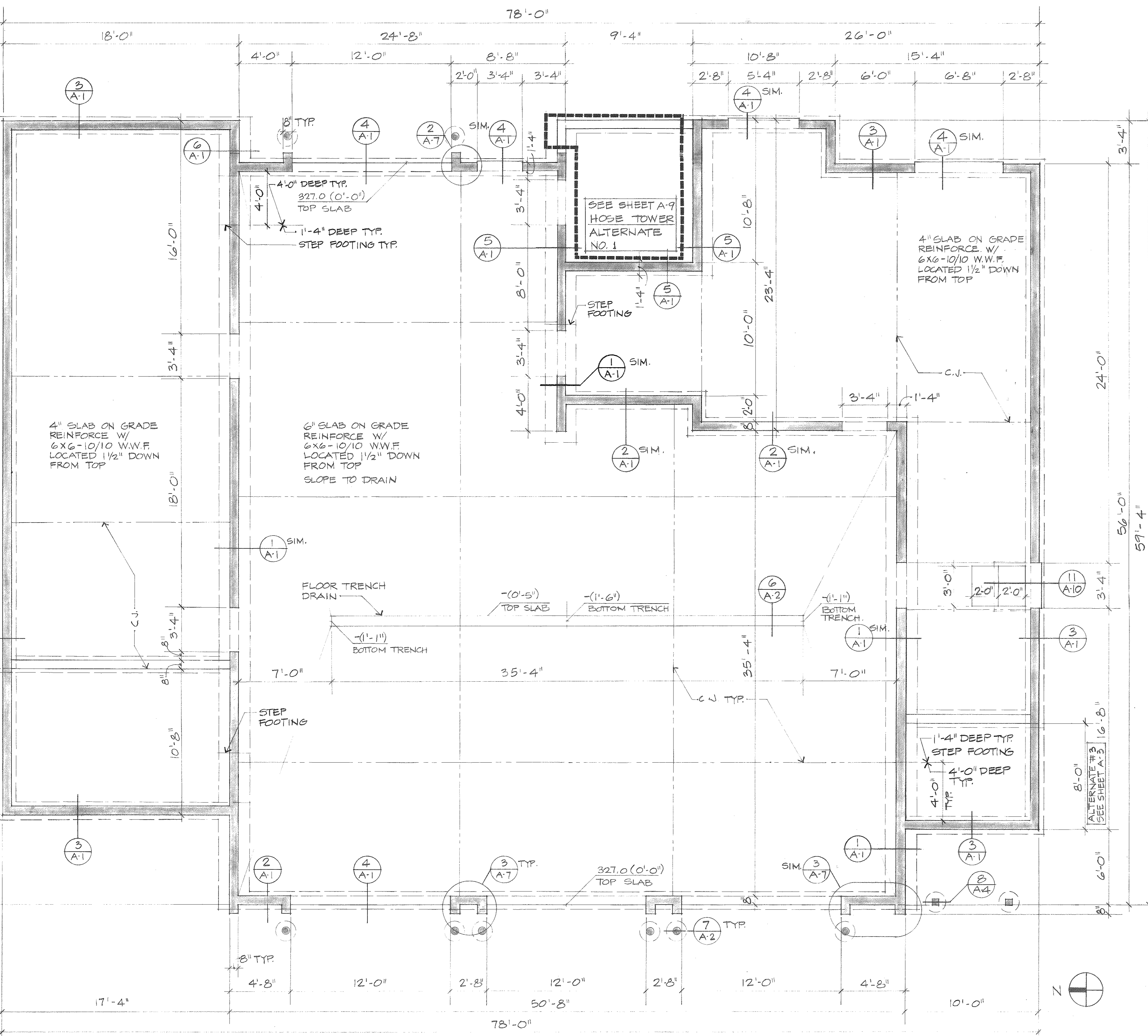
FOUNDATION PLAN
