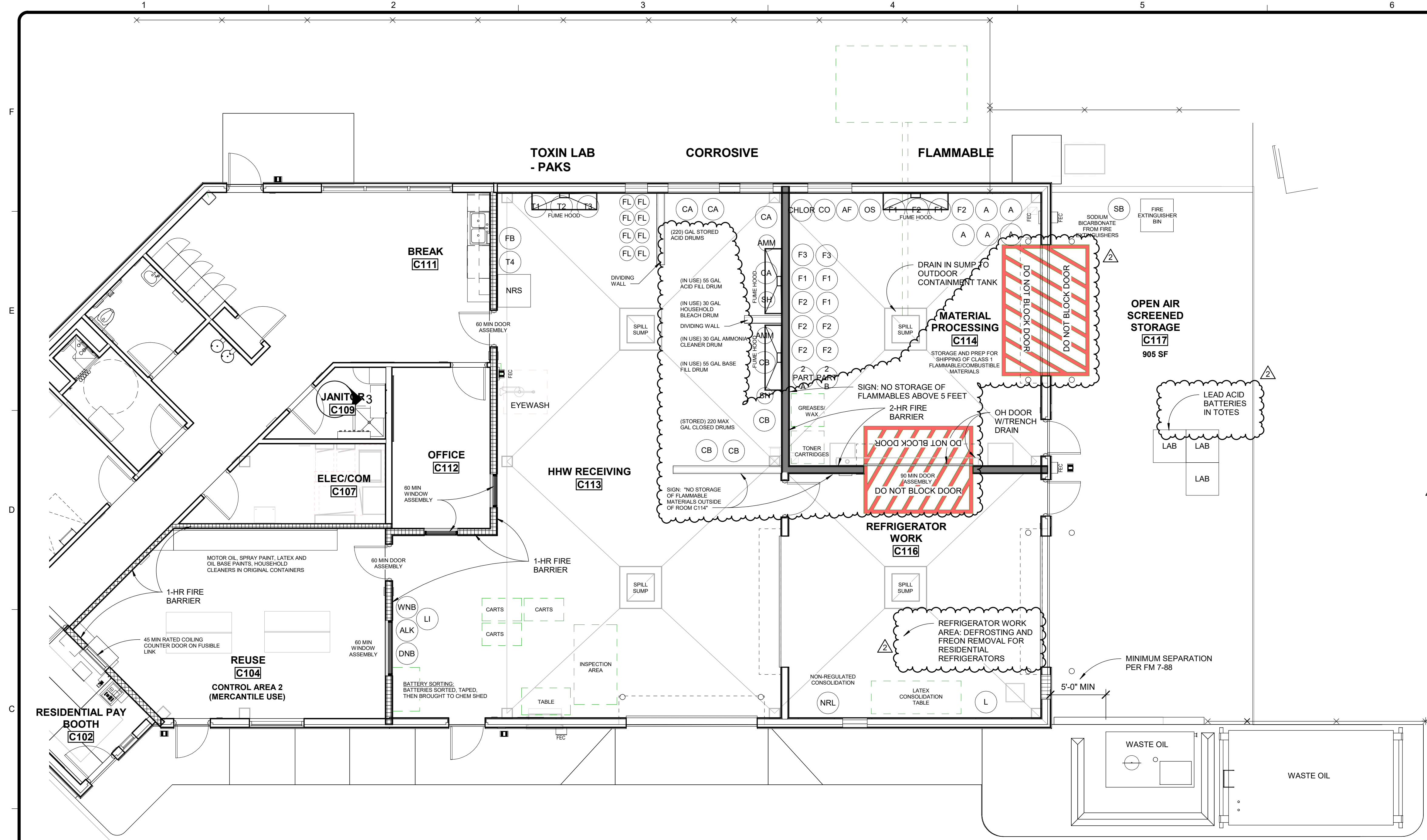
1 HAZARDOUS MATERIALS STORAGE PLAN AC801 SCALE: 3/16" = 1'-0"
