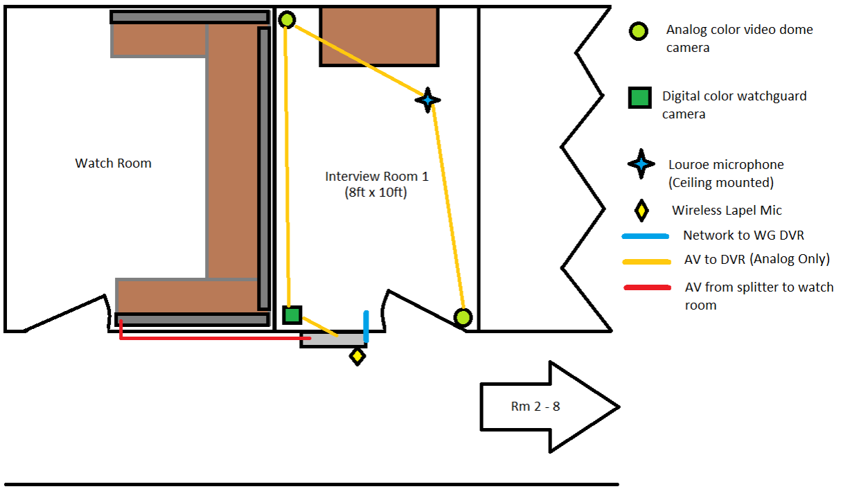
General Diagram of Interview Room Connections at HQ
